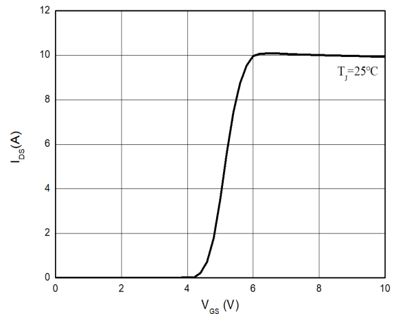
Figure 4. Typical Transfer Characteristics T_j = 25^\circ\text{C}
