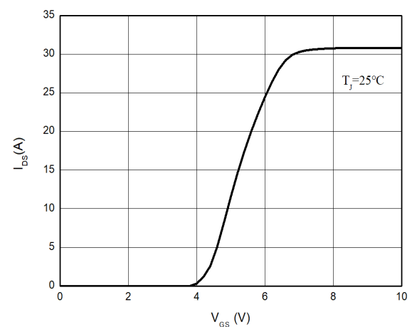
Figure 4. Typical Transfer Characteristics ( V_{ds} = 10\text{V} )
