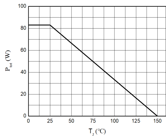
Figure 12. Power Dissipation
