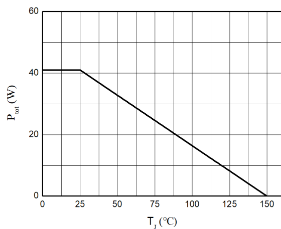
Figure 8. Power Dissipation
